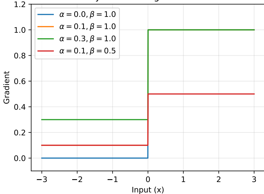
Leaky ReLU Surrogate Gradients
