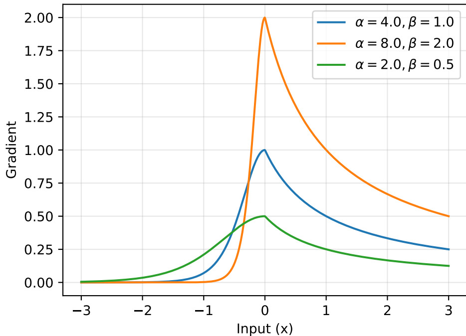
S2NN Surrogate Gradients
