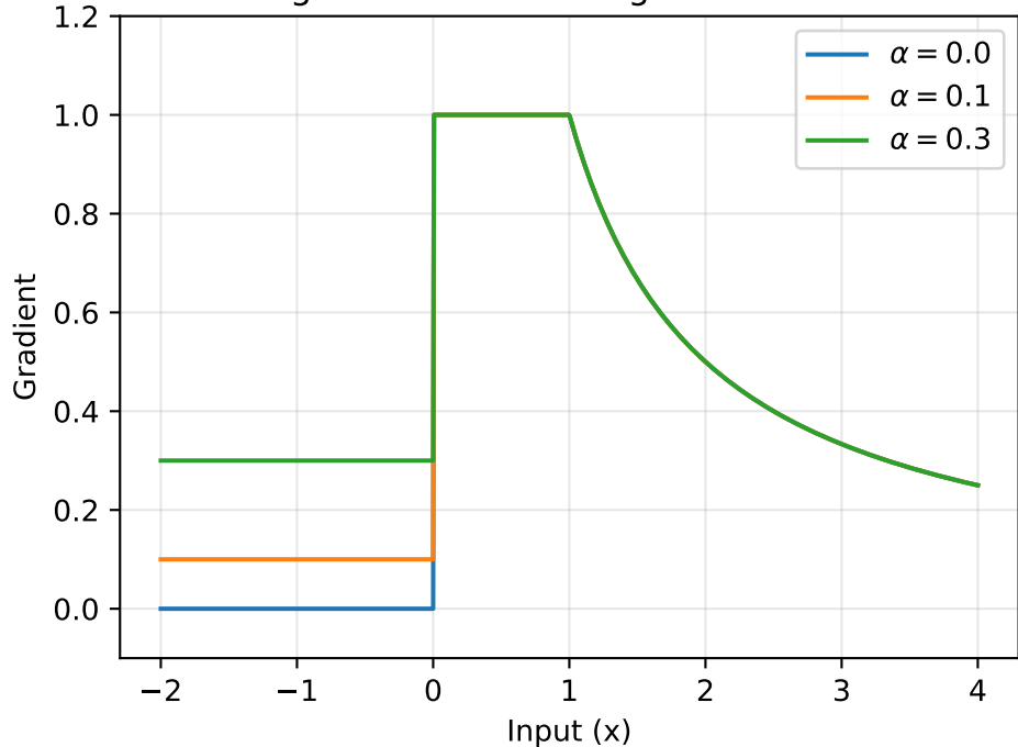
Log-tailed ReLU Surrogate Gradients
