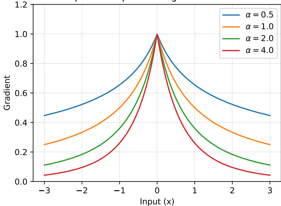
q-PseudoSpike Surrogate Gradients
